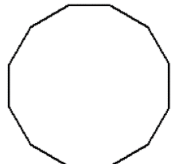
Regular Dodecagon
