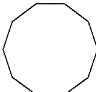
Regular Decagon
