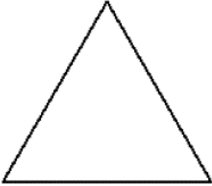
Equilateral triangle
