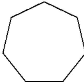
Regular Heptagon
