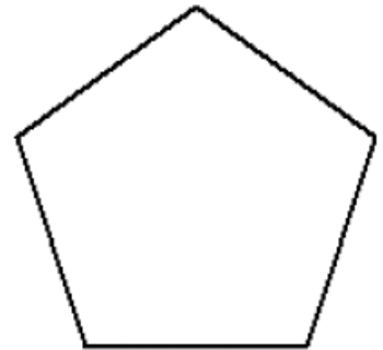
Regular Pentagon
